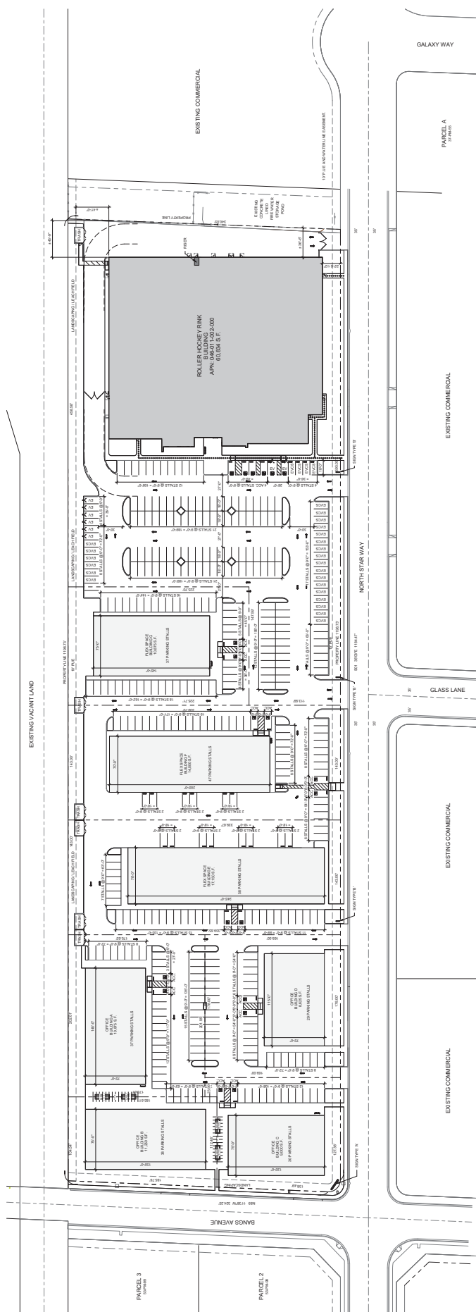
1 PROPOSED SITE PLAN 1" = 40'-0"
